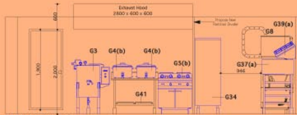
ELEVATION 2-2
