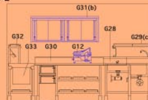
ELEVATION 5-5
