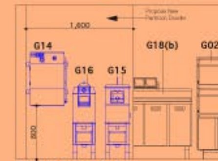
ELEVATION 4-4
