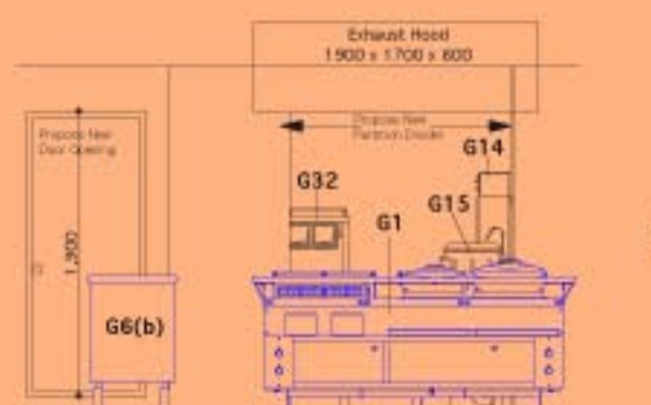
ELEVATION 8-8
