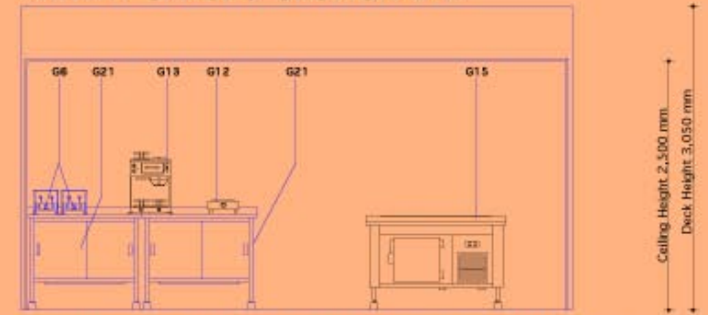
GALLEY ( Dishwash Area ) / SECTION 5-5
