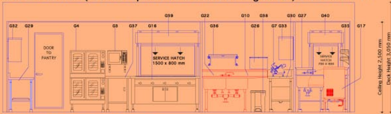
PANTRY SPACE / SECTION 3-3
