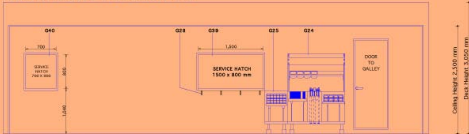
GALLEY SPACE ( Hot Cooking Area ) / SECTION 4-4
