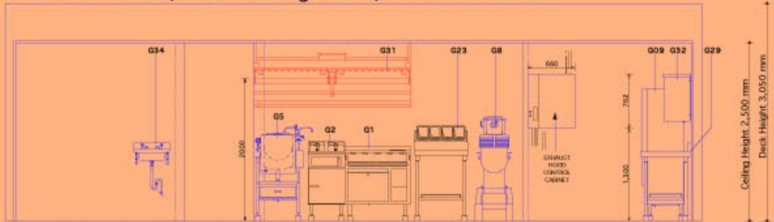
GALLEY & PANTRY SPACE / SECTION 7-7
