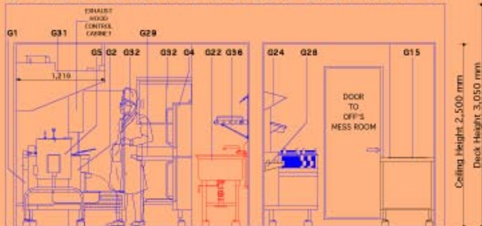
GALLEY & PANTRY SPACE / SECTION 7-7
